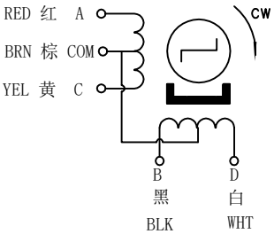
接线图 COLOURS OF LEAD WIRES
