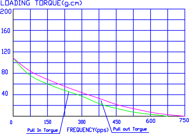
PULSE-TORQUE CHARACTERISTICS
