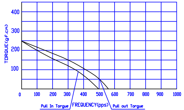
PULSE-TORQUE CHARACTERISTICS
