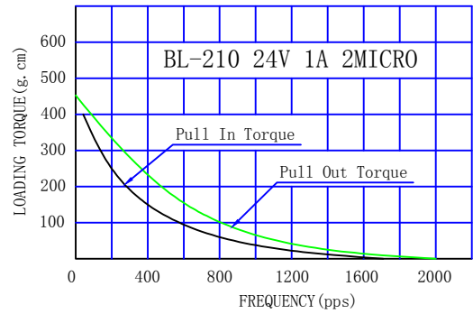
□ PULSE-TORQUE CHARACTERISTICS
